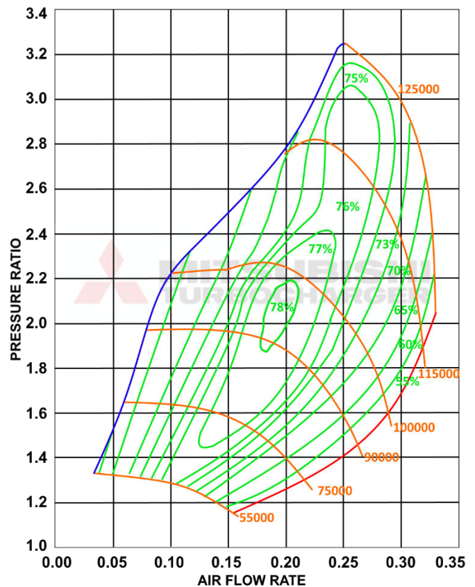
COMPRESSOR MAP
