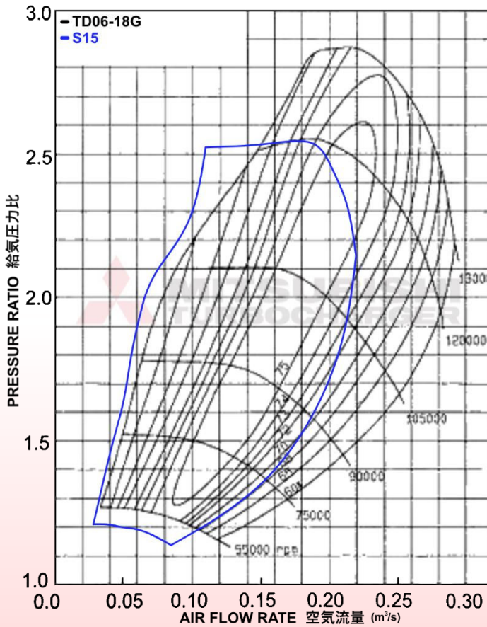
COMPRESSOR MAP
