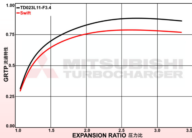
TURBINE MAP
