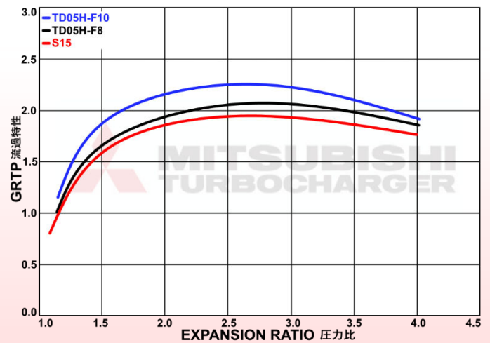
TURBINE MAP
