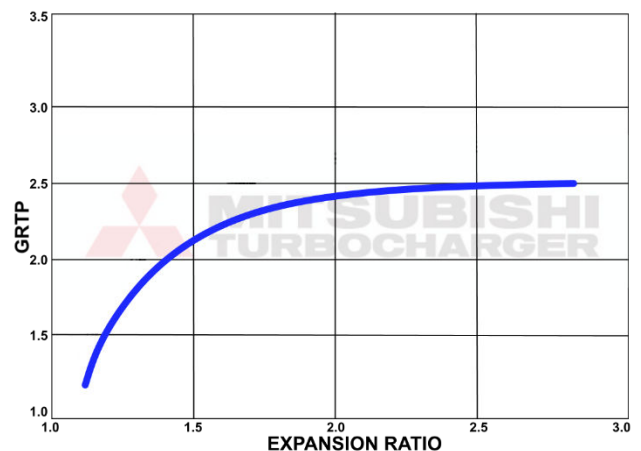
TURBINE MAP
